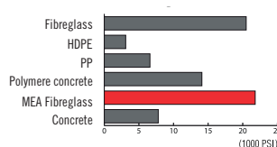
Compression resistance
